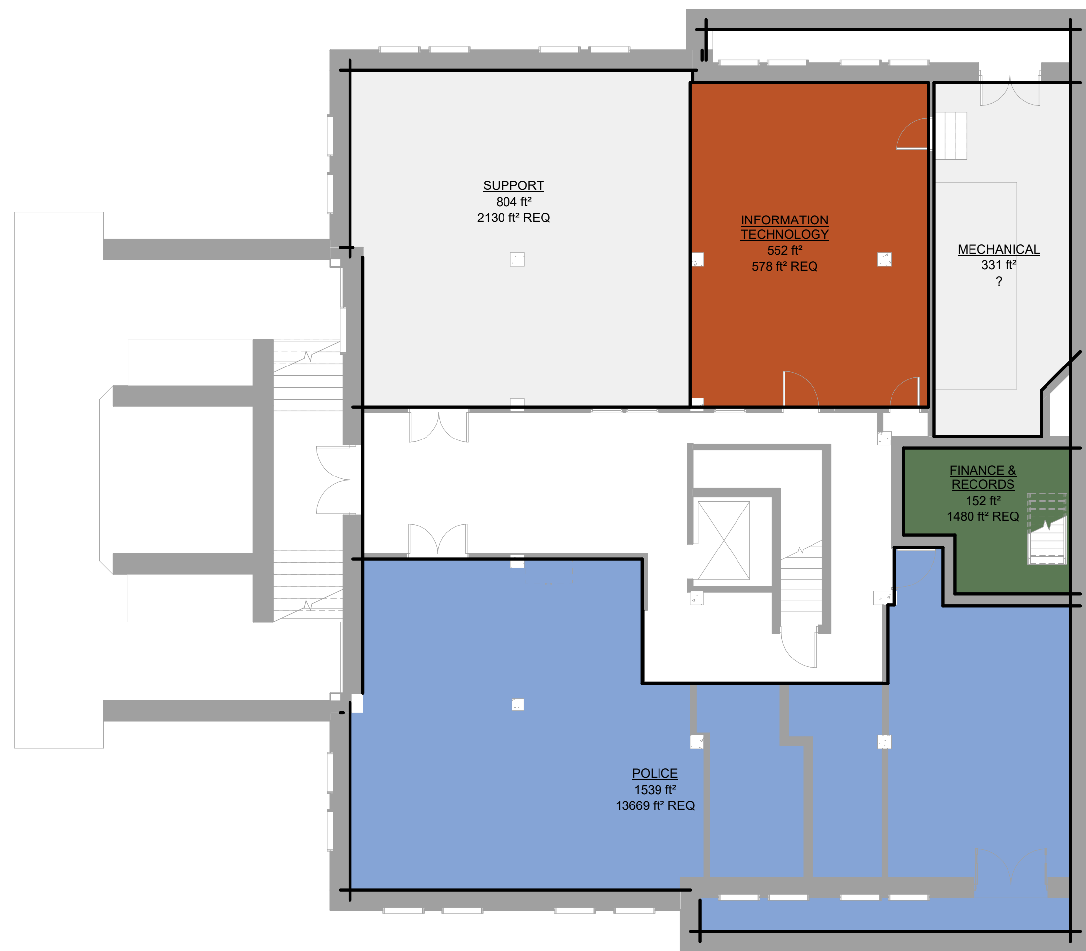
BASEMENT 1/8" = 1'-0"
